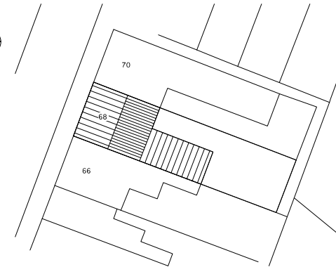
EXISTING SITE PLAN 1:200
